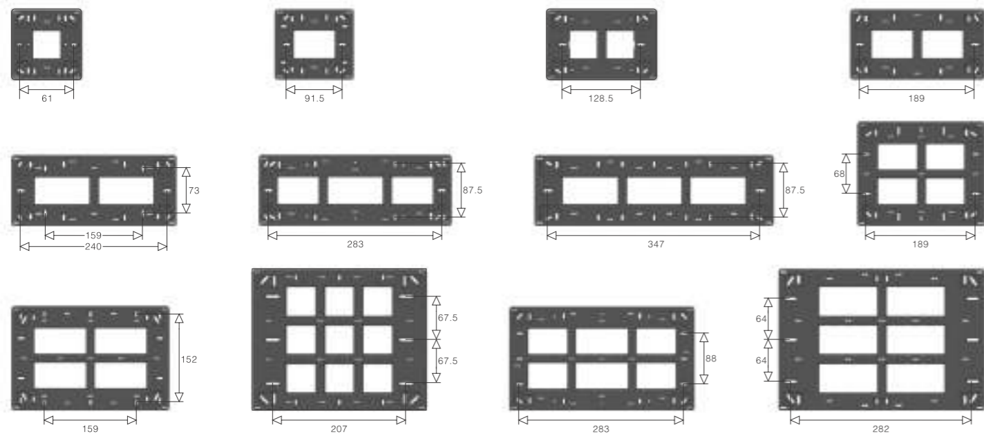
F-WOOD MOUNTING FRAMES - HORIZONTAL & VERTICAL DISTANCE FOR SCREWING (dimensions in mm)
