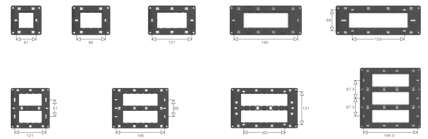
FLARE MOUNTING FRAMES - HORIZONTAL & VERTICAL DISTANCE FOR SCREWING (dimensions in mm)
